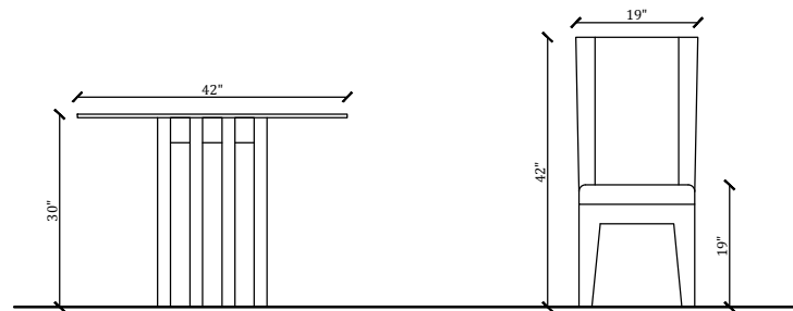
SIDE VIEW OF DINING TABLE
