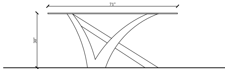
DINING TABLE FRONT VIEW
